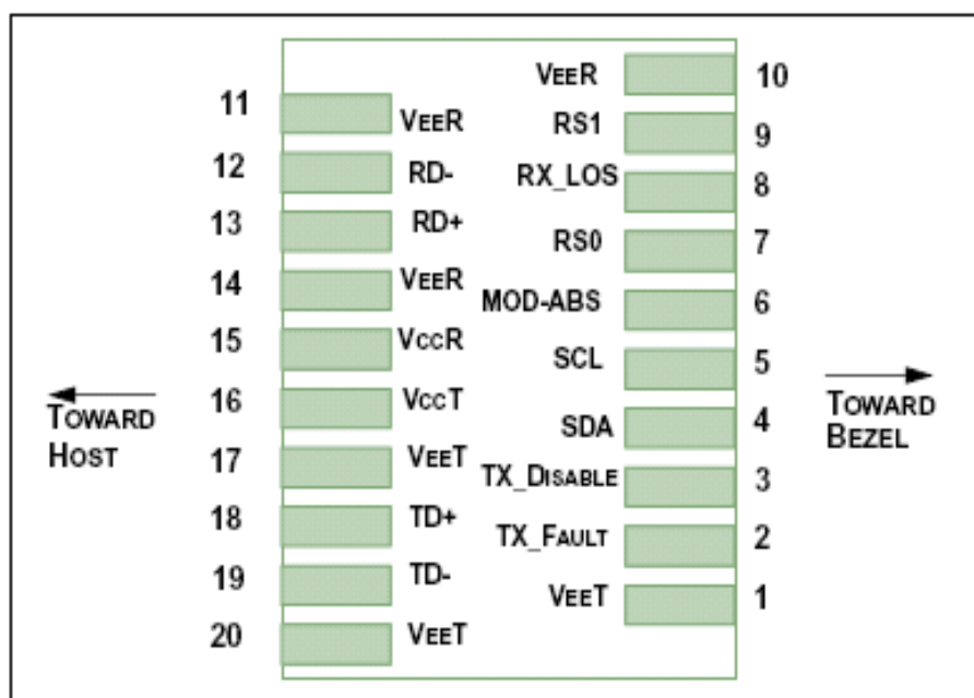
Pin Definitions
